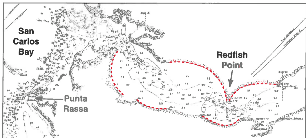
Figure 23. Drowned River Valley features.
