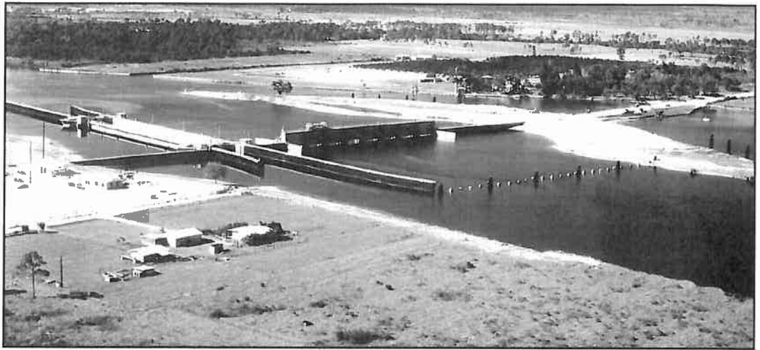
Figure 10. W.P. Franklin Lock, 1968.
