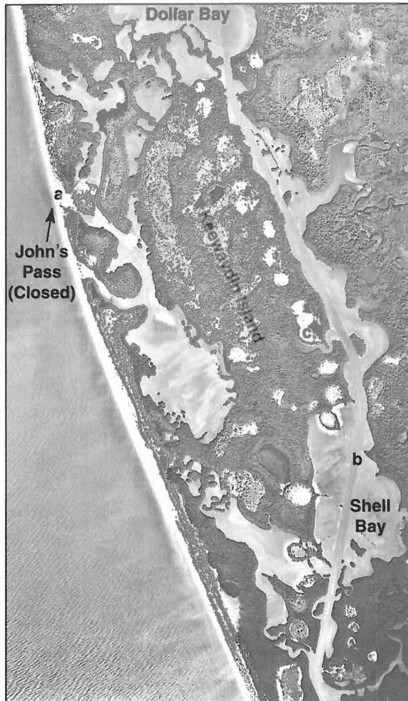
Figure 9B. Shell Bay and John's Pass, 1940s.
