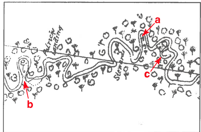
Figure 22. Meanders in the Caloosahatchee, 1887.
