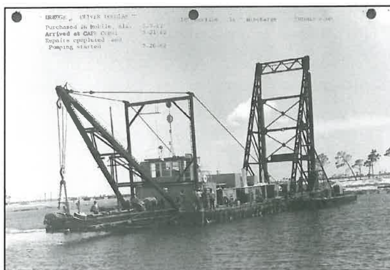
Figure 6. Dredge Oliver Douglas, 1962.
