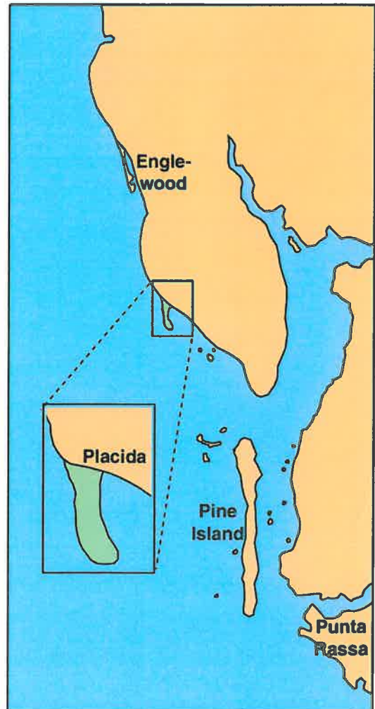
Figure 5. Charlotte Harbor shoreline approximately 5000 years ago.
